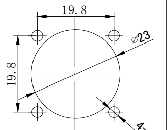
TYPICAL PANEL CUTOUT
