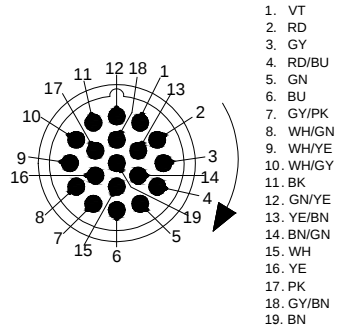
MALE END VIEW
